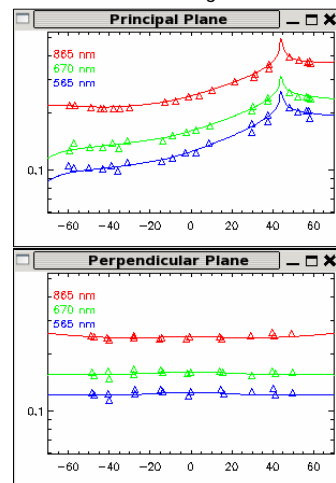
Measured (symbols) and modeled (lines) reflectances in the principal and perpendicular planes for the selected wavelengths. The Y axis can be either on a linear or a log scale.
